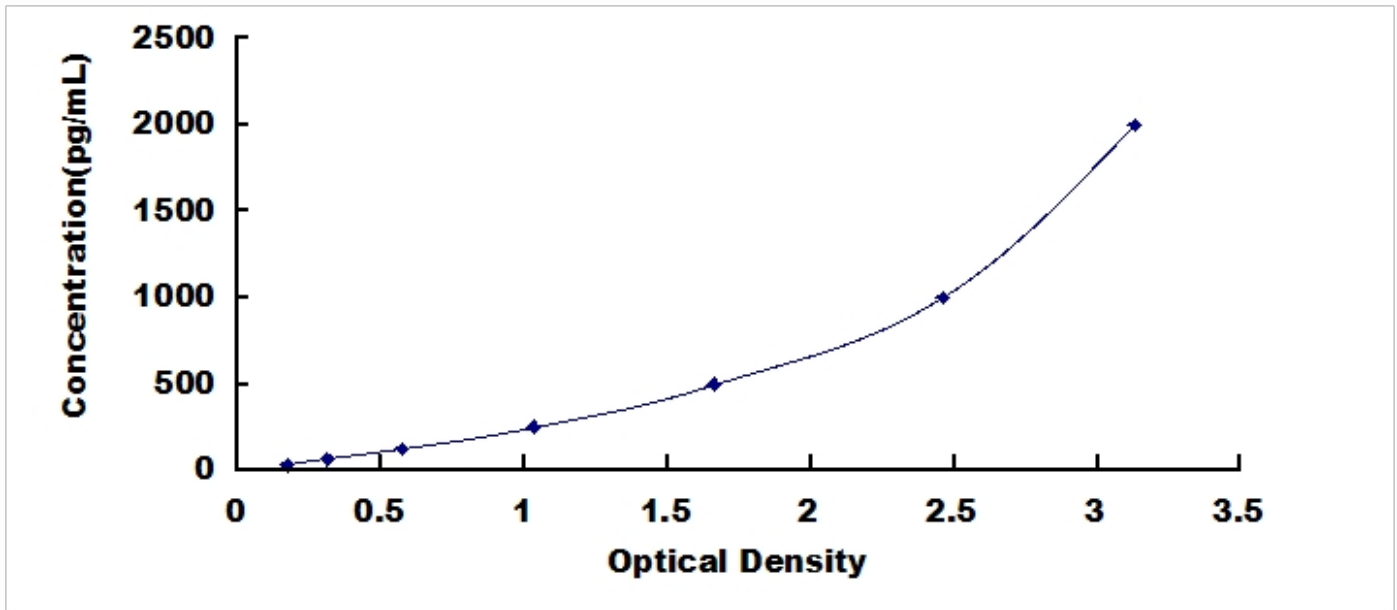
Typical Standard Curve for NGF, Rabbit ELISA.
